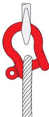
Avoid side loading and place sling eye on shackle body
