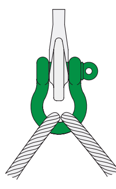
Slings should be in bowl of shackle (do not use chain / Dee shackles) 120 deg sling angle is max
